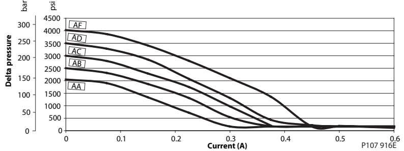
P4, Relief pressure vs. current
