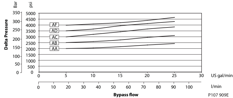
P1 and P3 valve settings, (low flow)
